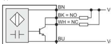
(i)DOL 27 NPN
